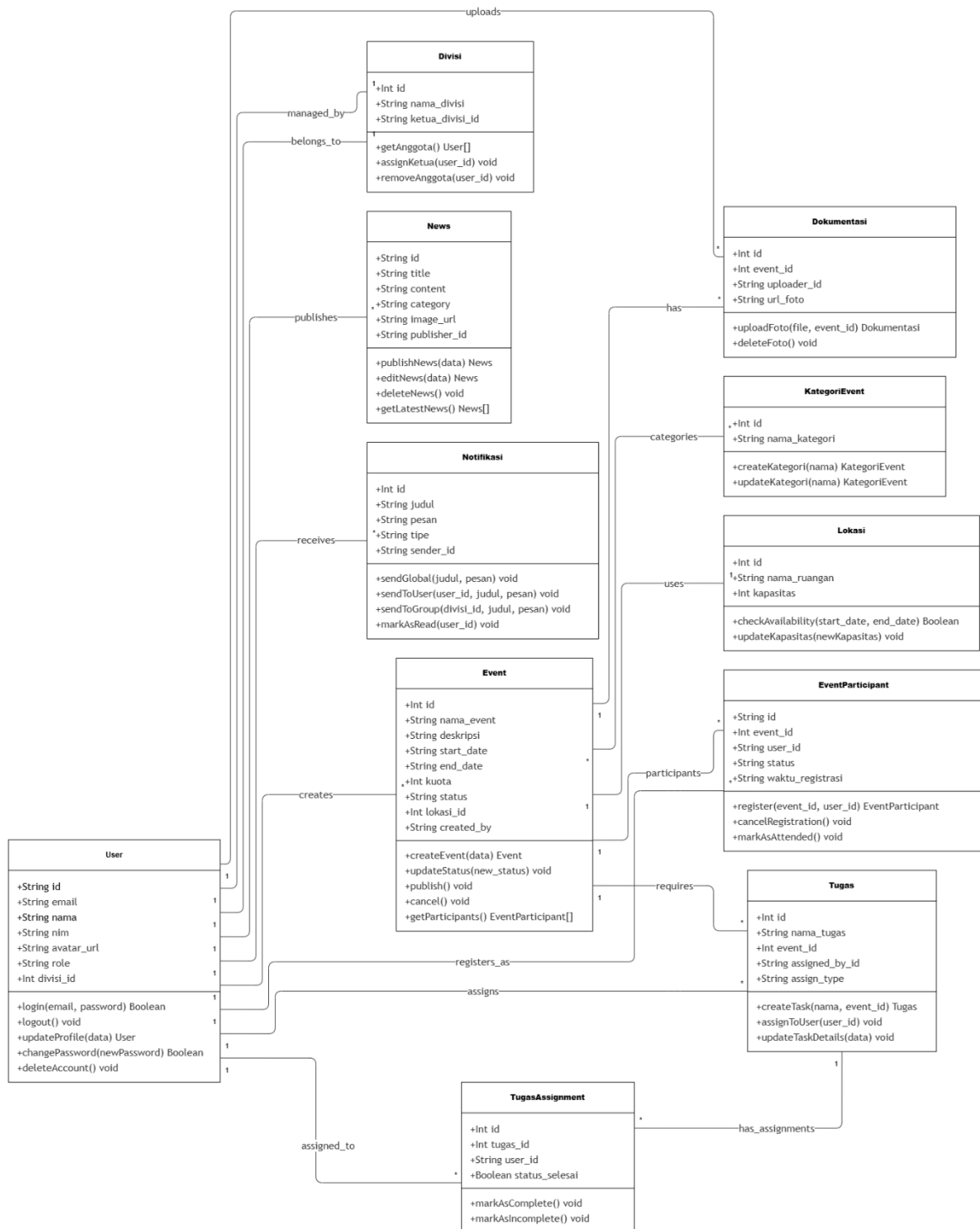
Gambar 4.2 Class Diagram
